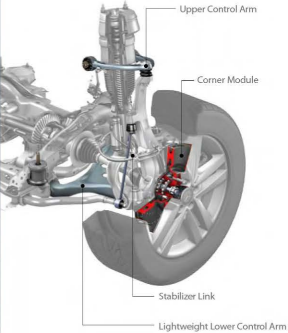
Lightweight Lower Control Arm
